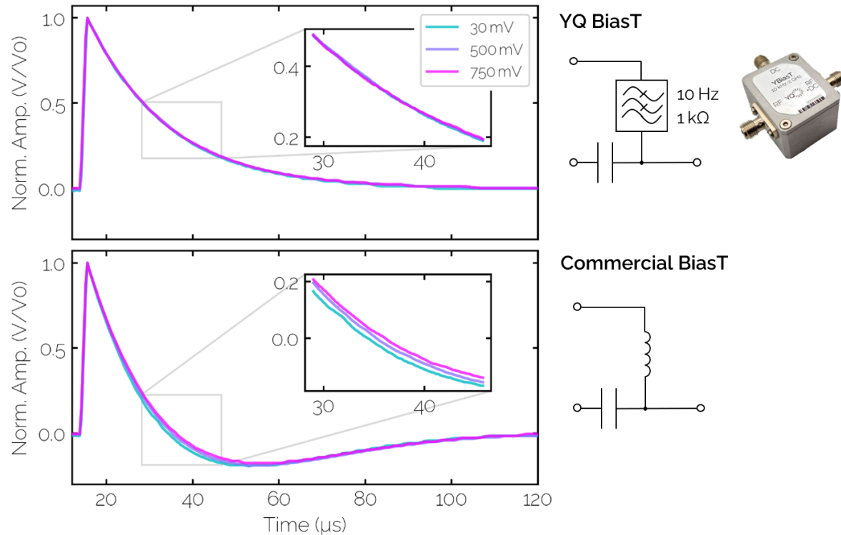
Figure 3 Step response of the BiasT into a 50\ \Omega load for (top) the YQ BiasT and (bottom) a commercially available BiasT. The step response is measured for different pulse amplitudes V_0 , given in the inset in the upper graph, and the normalized responses are shown.
