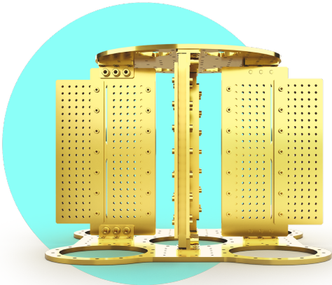
Cryo Coldstage OFHC copper with gold-plating
