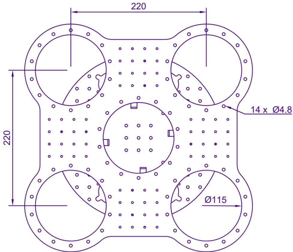
Drawing Coldstage – Bottom View [mm]
