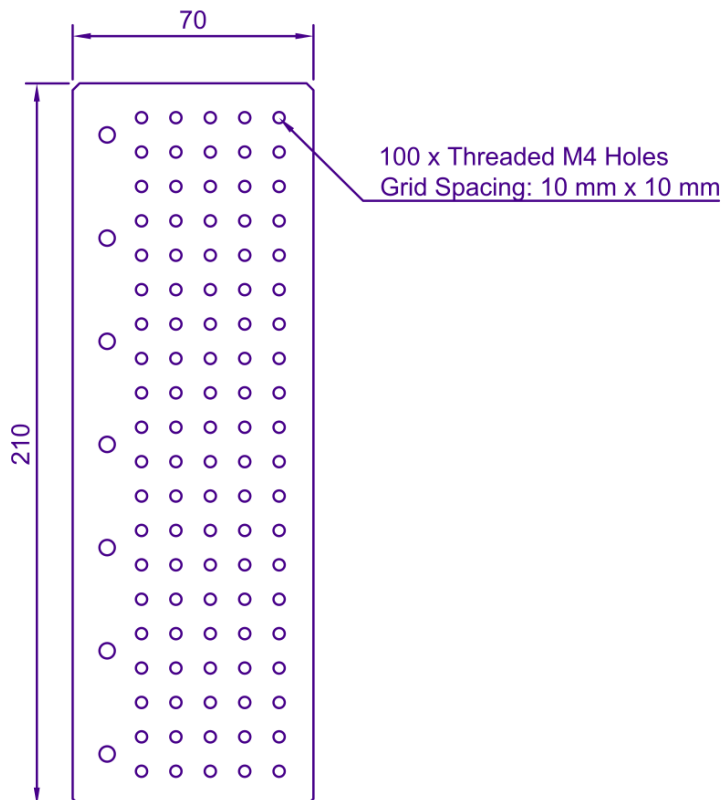
Drawing Breadboard – Side View [mm]
